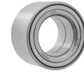
ZEN-90020 DIANTEIRA S/ABS 49X84X48 MASTER 2.5 03>13 2.8 02>06
